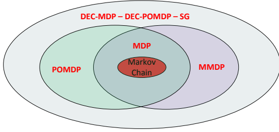
Fig. 2. Extensions of Markov decision models.
