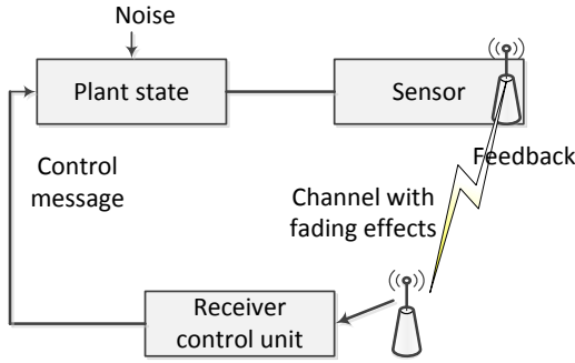
Fig. 5. System architecture of the closed loop control system tackled in [64].
