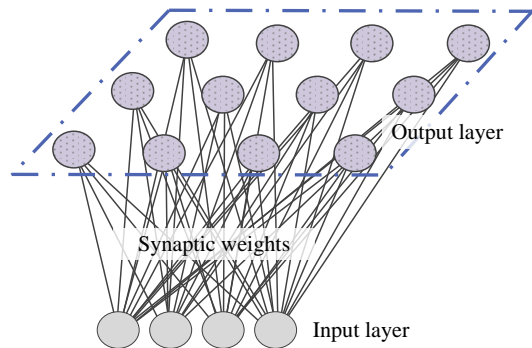
Fig. 16. A self organizing map with a 4D input space that is mapped to 12 distinctive classes in a 2D output lattice. Synaptic connections are tuned using an offline competitive learning over historical data.
